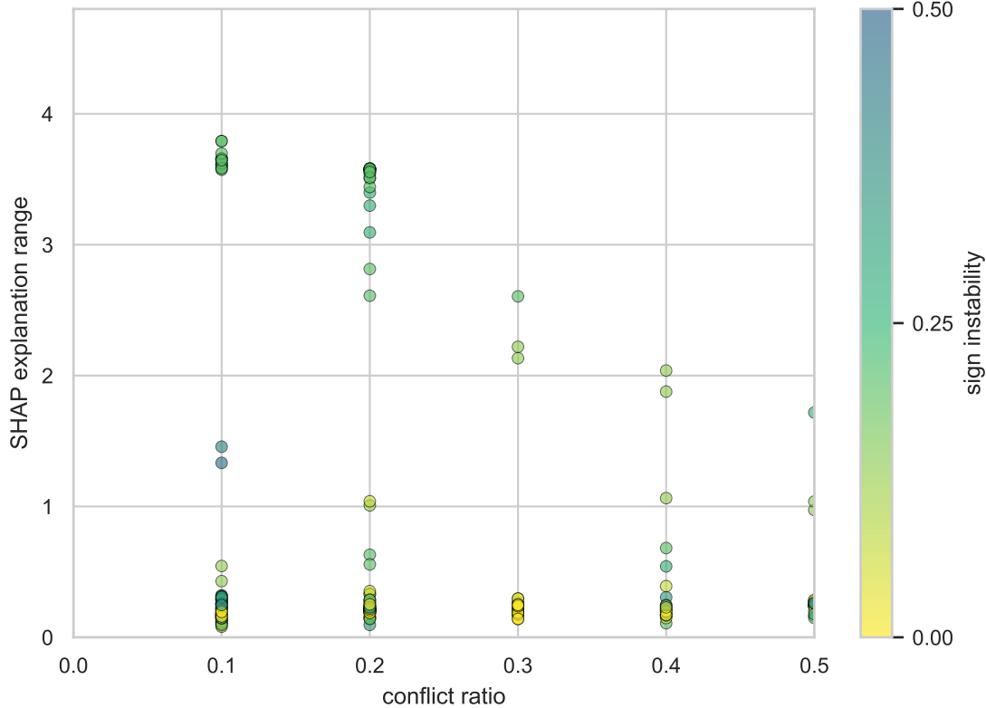
num__srv_count: SHAP explanation range (Spearman r = 0.033 )
